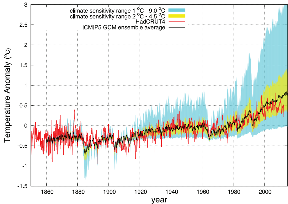
Figure 2: HadCRUT4 GST record (red) vs. the CMIP5 (rcp60) ensemble mean simulation (black). Uncertainty ranges refer to equilibrium climate sensitivity to CO_2 doubling spanning 2-4.5 °C (yellow), and 1-9 °C (cyan).
