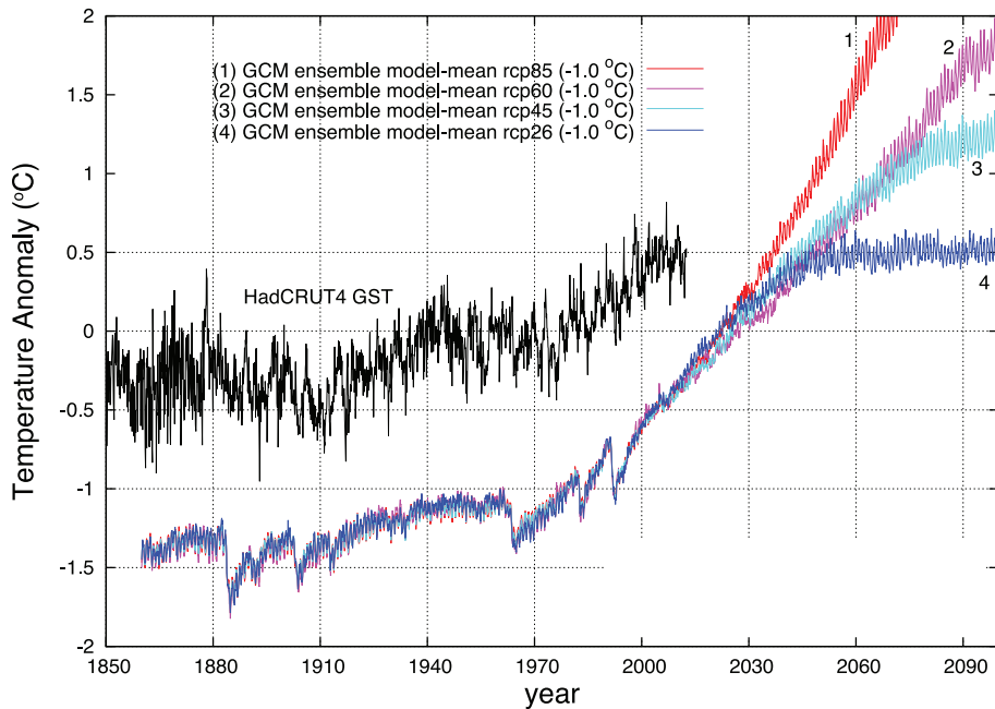
Figure 1: HadCRUT4 (1850-2012) GST (black) [1]. Four Coupled Model Inter-comparison Project 5 (CMIP5) GCM ensemble mean simulations based on known historical forcings (1860-2006) and four alternate 21 st century emission projections (records are shifted by 1 °C for visualization).
