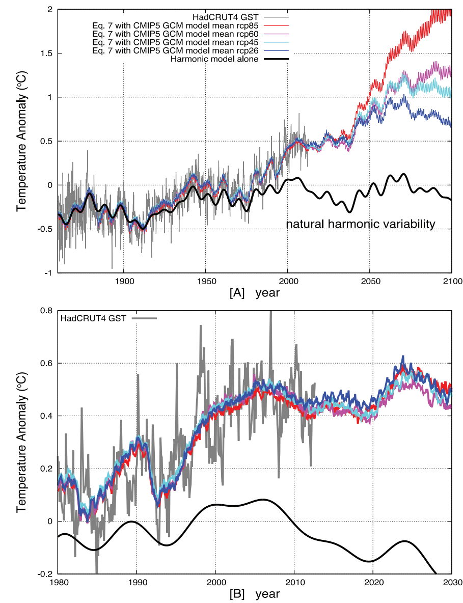
Figure 16: [A] HadCRUT4 GST (gray) superimposed on the empirical climate model given by Eq. 7 where the anthropogenic/volcano component M_{A,V}(t) is derived from the four alternate CMIP5 GCM ensemble average simulations of Fig. 1. The smooth black curve corresponds to the six-frequency harmonic component alone, representing the modeled natural variability. [B] Zoom of [A] for 1980 to 2030.
