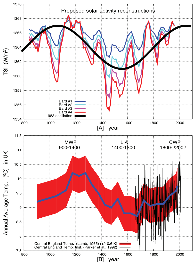
Figure 3: [A] Proposed solar activity reconstructions based on the solar proxy records of 10 Be and 14 C cosmogenic isotope production [50]. [B] Central England: HadCET temperature record (black) [48] superimposed on a proxy temperature reconstruction (red) [49].
