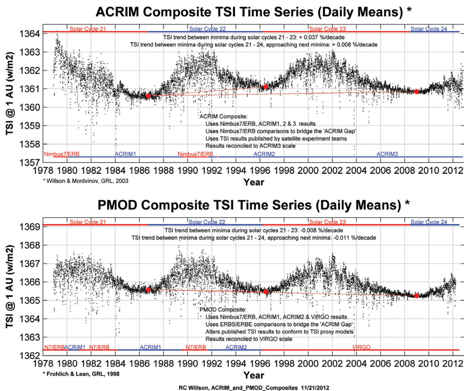
Figure 14: (Top) ACRIM total solar irradiance satellite composite [113]. (Bottom) PMOD total solar irradiance composite [111].
