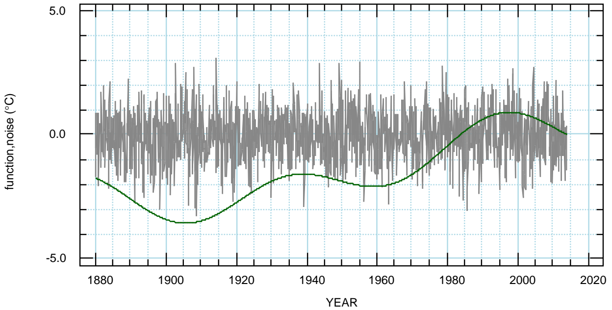
sine+cos+line+noise
