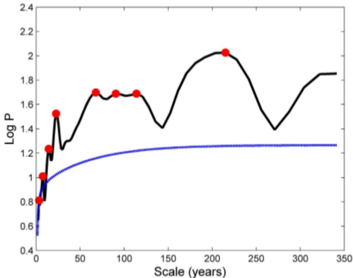
Figure 3. The time-averaged power spectrum of the driving force.
