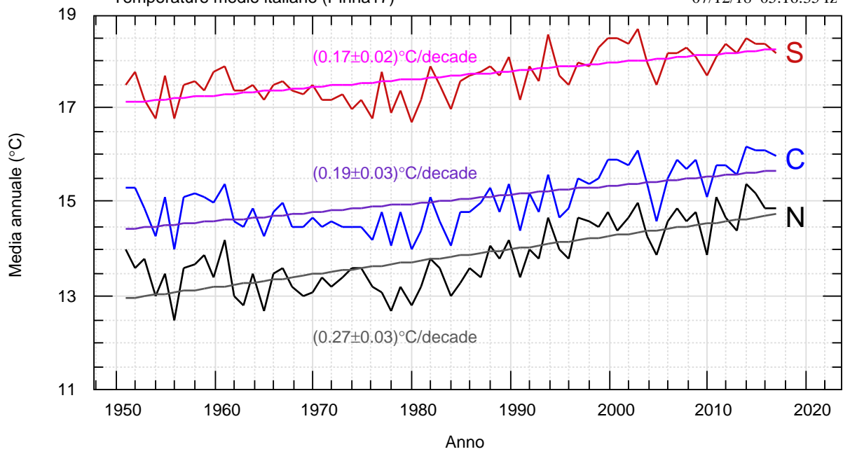
Temperature medie italiane (Pinna17)
